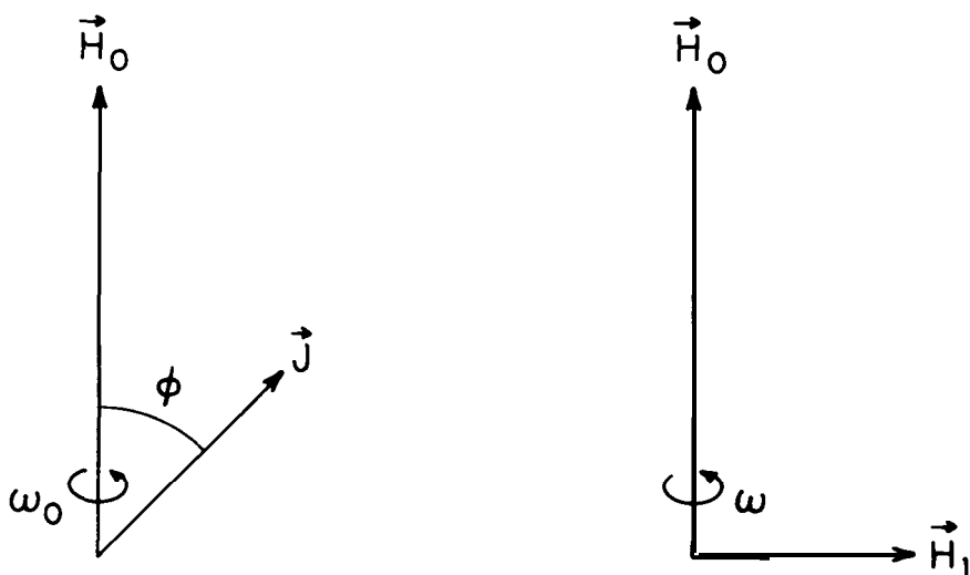
Figure 3. Precession of the nuclear angular momentum J (left) and the rotating magnetic field H_1 (right) in the Rabi method.
